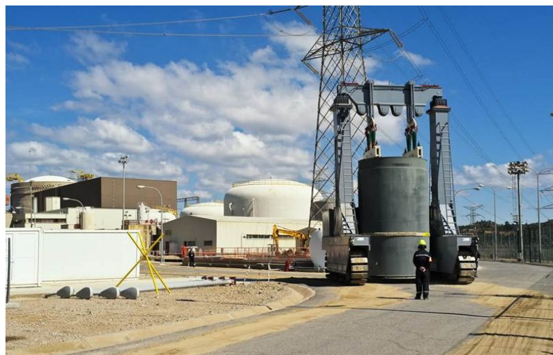
Transport of spent fuel cask to the Ascó nuclear power plant ITS facility.
